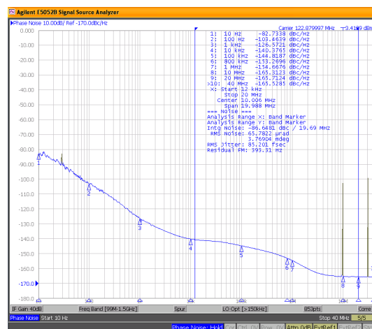
Figure 8.3. Typical Phase Noise and Jitter—122.88 MHz
