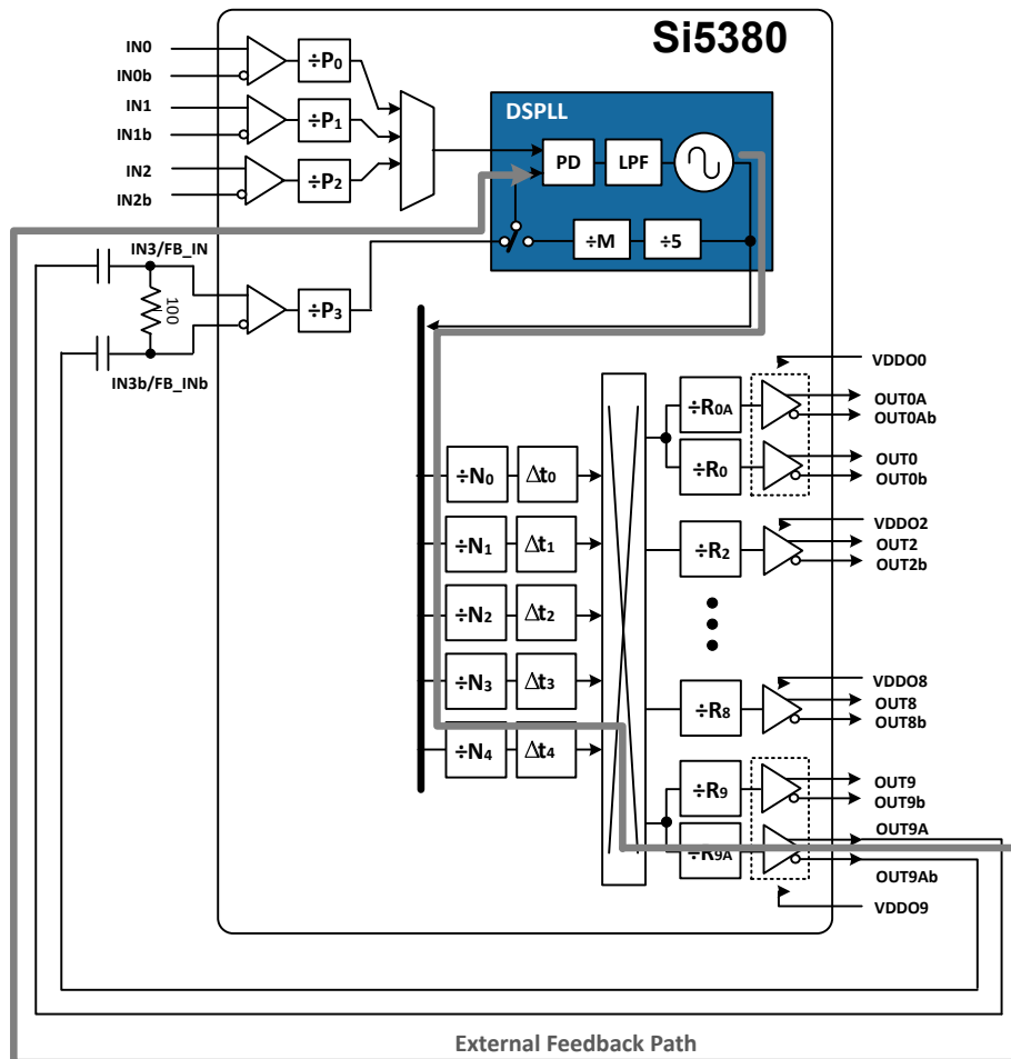
Figure 3.6. Si5380 Zero Delay Mode Set-up
