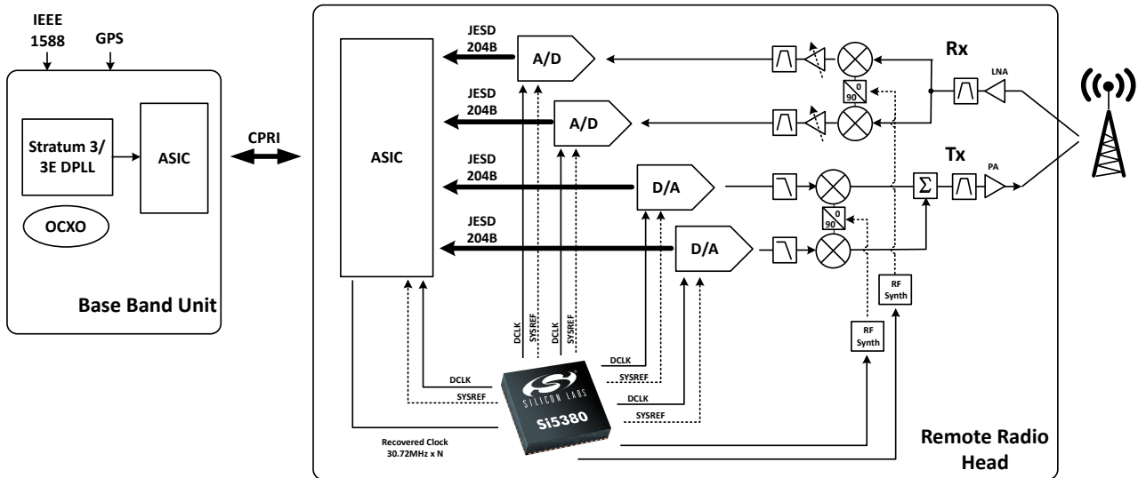
Figure 6.2. LTE Base Station Using JESD204B Data Converters
