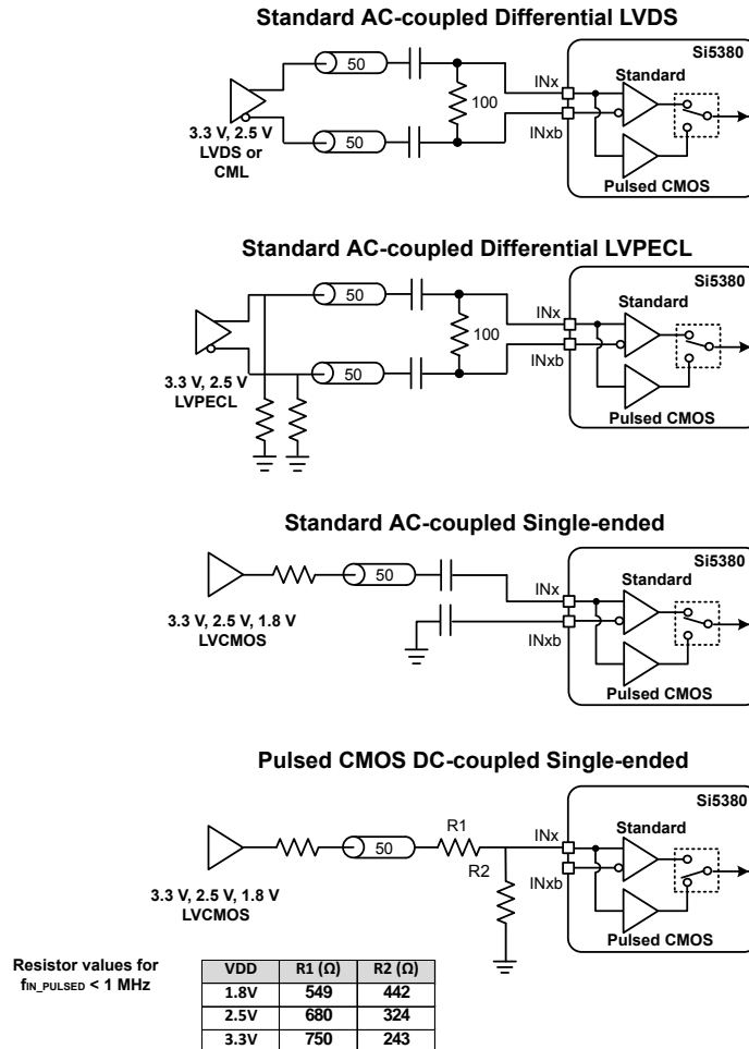
Figure 3.5. Termination of Differential and LVCMOS Input Signals
