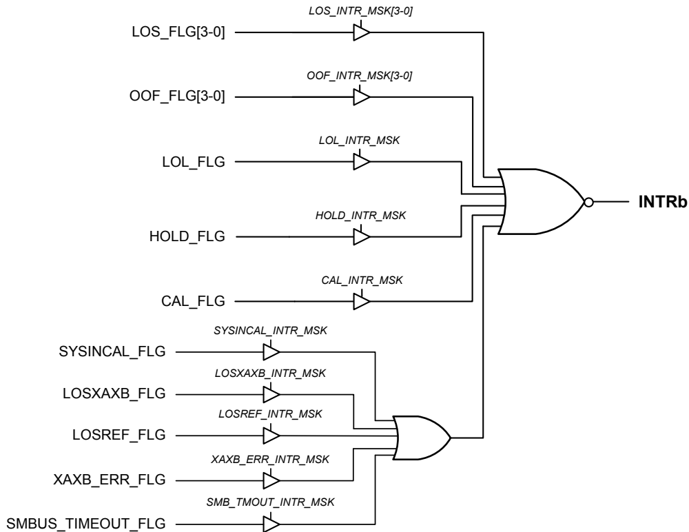
Figure 3.13. Interrupt Triggers and Masks
