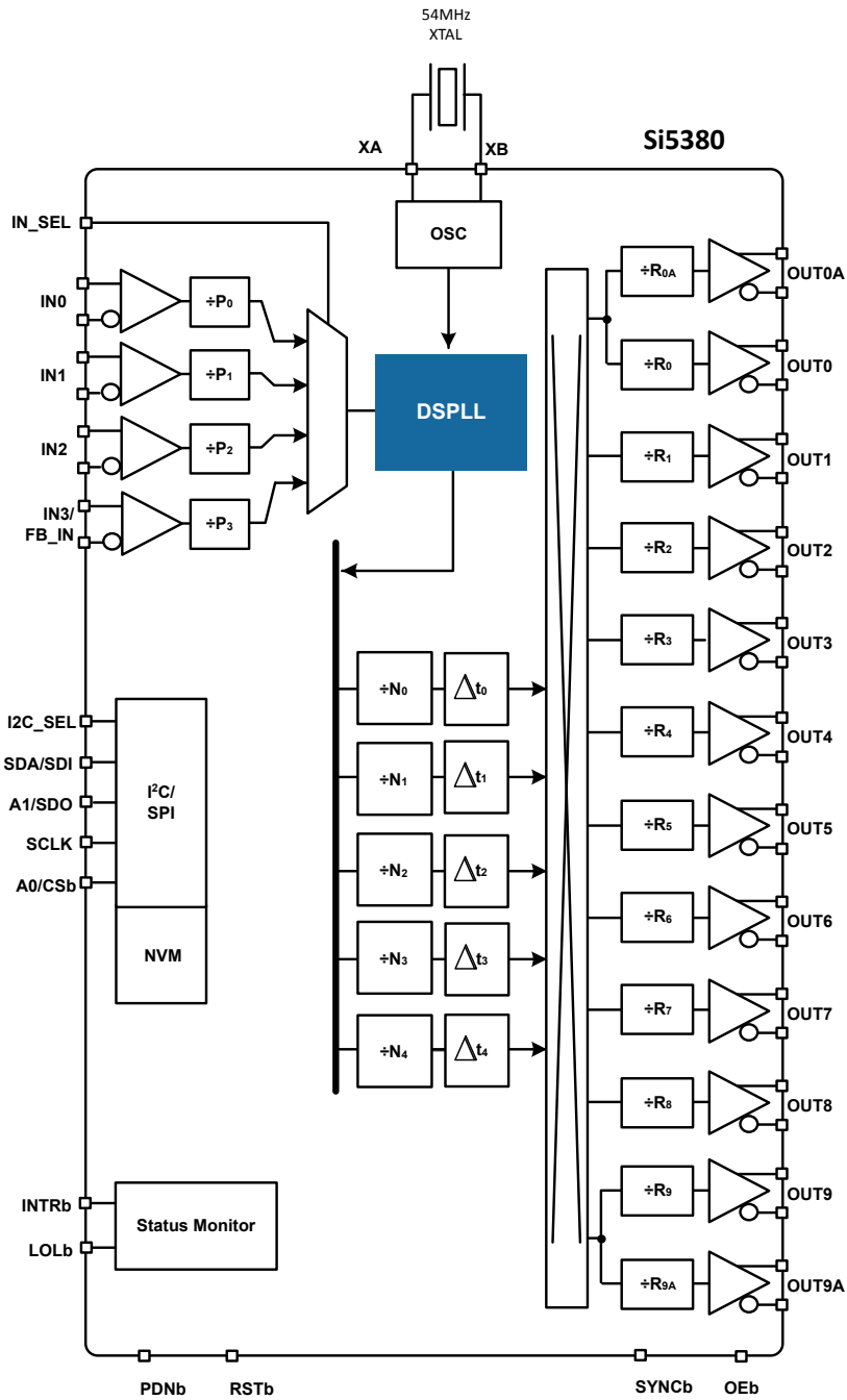
Figure 7.1. SI5380 Block Diagram
