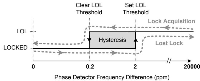
Figure 3.12. LOL Set and Clear Thresholds
