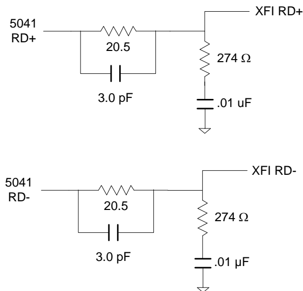
Figure 8. EVB De-Emphasis Circuit
