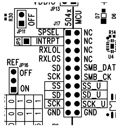
Figure 5. External MCU
